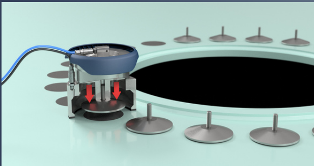
Bonding of C-Claw around the hatch
